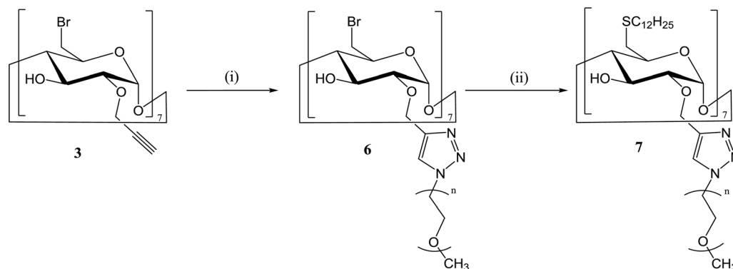
Scheme 2 Synthesis of the pegylated cyclodextrin 7 (i) 1-azido-1-deoxy- \omega -methoxy-PEG 500 , CuSO 4 , 5H 2 O, sodium ascorbate, DMF–H 2 O, 80 °C (ii) dodecanethiol, NaH, 80 °C.
