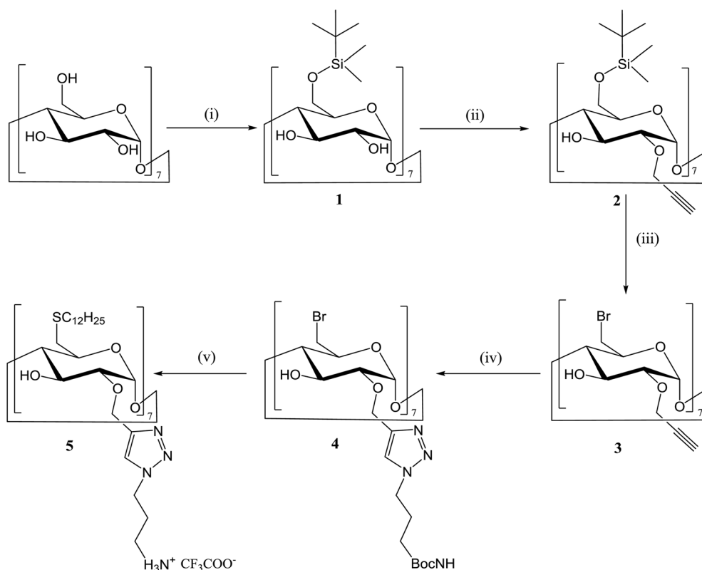
Scheme 1 Synthesis of the cationic cyclodextrin 5 (i) TBDMSCl, pyridine, 88% (ii) propargyl bromide, NaH, DMF (iii) PPh 3 , Br 2 , CH 2 Cl 2 , (iv) tert -butyl 3-azidopropylcarbamate, CuSO 4 ·5H 2 O, sodium ascorbate, DMF–H 2 O, 80 °C (v) (a) dodecanethiol, NaH, 80 °C, (b) TFA, CH 2 Cl 2 .
