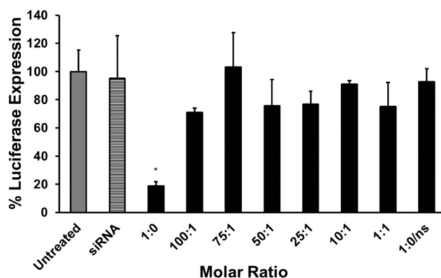
Fig. 4 Effects of molar ratio of cationic CD 5 to pegylated CD 7 on silencing of luciferase reporter gene expression in Caco2 cells at mass ratio cationic CD 5:siRNA = 10. Results are expressed as Mean \pm S.E. M. ( n = 3 ). * p < 0.05 relative to untreated cells.
